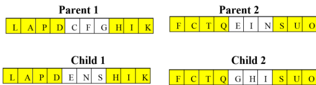
Figure 4. OX Crossover operator using only one wheel.
